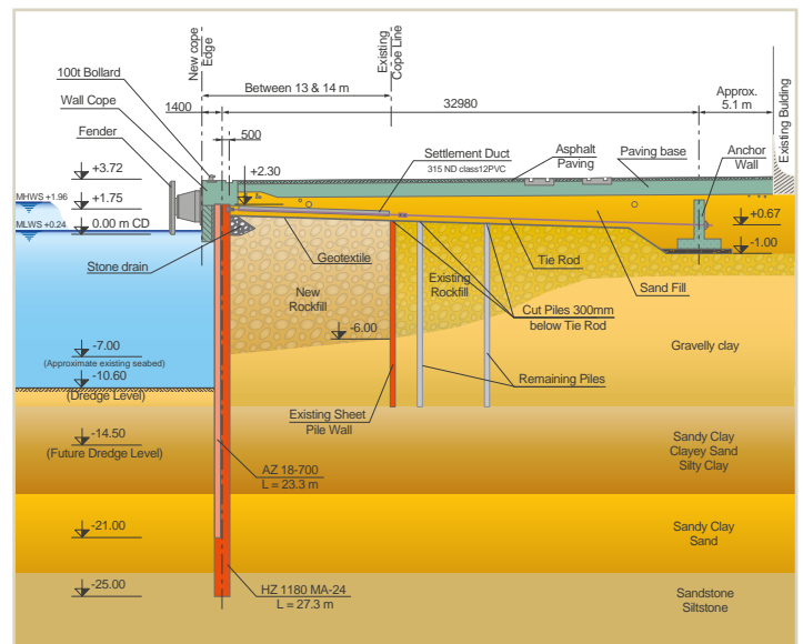
Preliminary design for a quay wall
